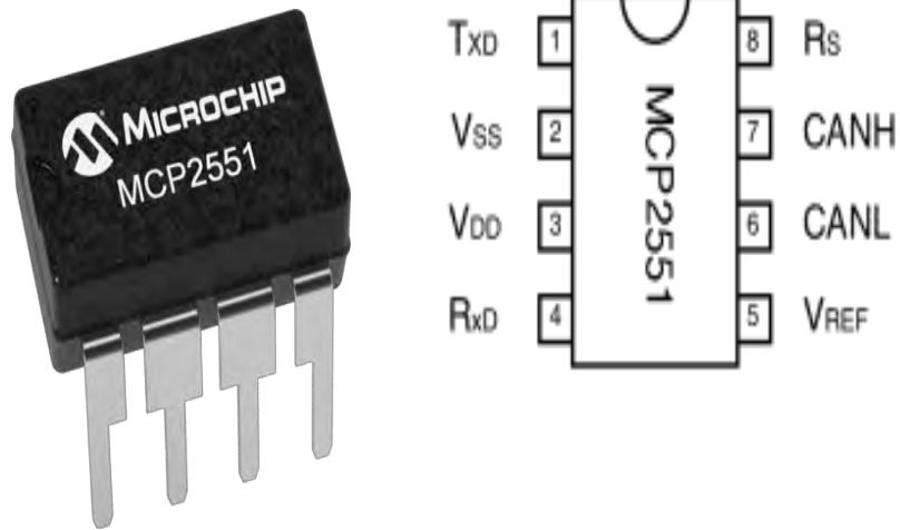
Figure 3.3 MCP2551 IC
