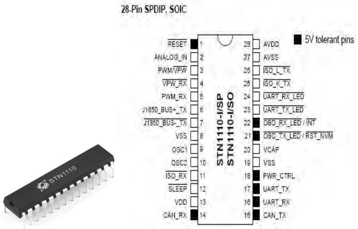
Figure 3 .1 STN1110 IC Pin Configuration
