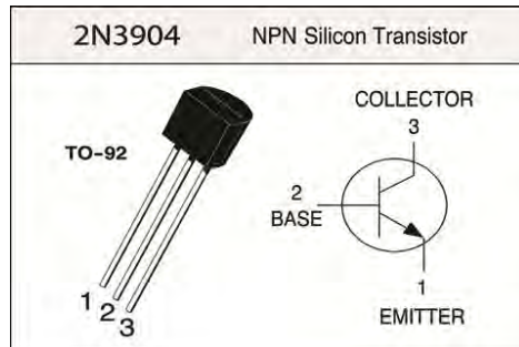
Figure 3.7 2N3904 Transistor
