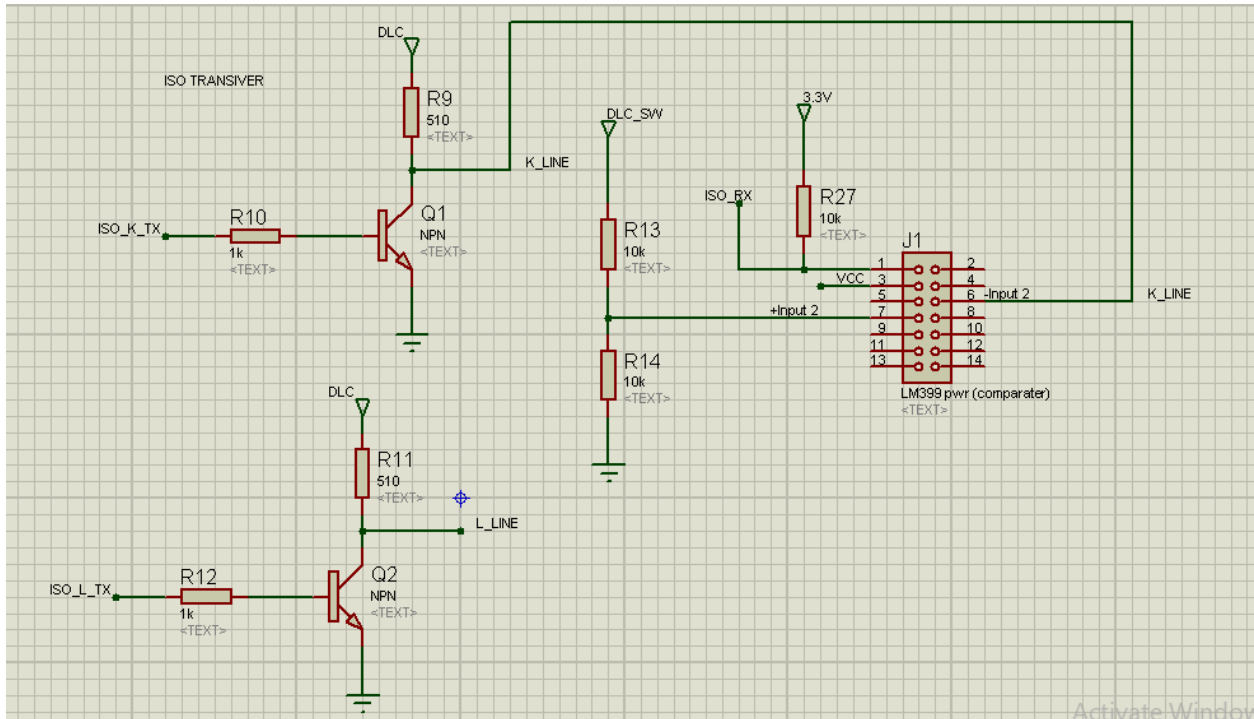
Figure 3.11 ISO_Transiver Diagram
