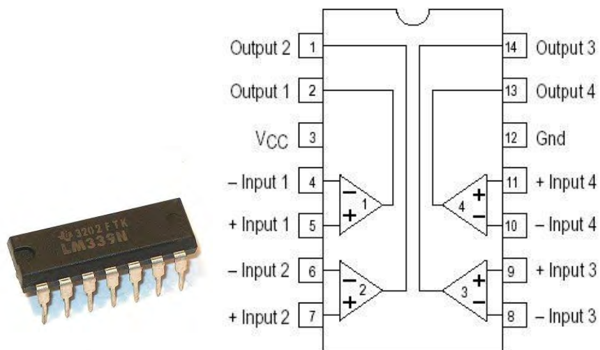
Figure 3.1 LM399PWR
