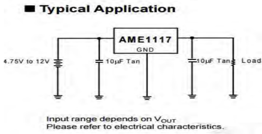
Figure 3.5 AME1117 (3.3V Voltage Regulator)
