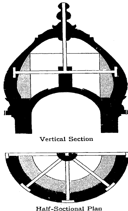
DIAGRAM SHOWING CONSTRUCTION OF LOTUS DOME
